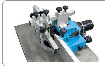
Guide with horizontal and vertical pressers
