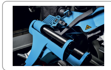
Head with radial sliding
