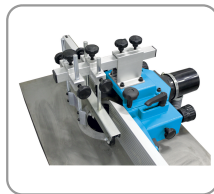
Guide with horizontal and vertical pressers
