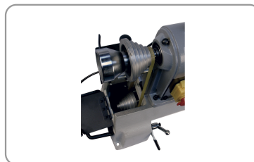
6 spindle speeds
