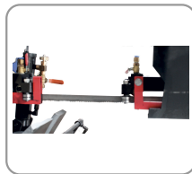
Adjustable and highly precise blade guide with 8-point bearings
