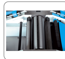
Driving rollers Ø 40 mm, 95 mm cutterblock with 4 blades
