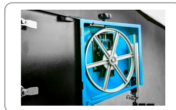
Balanced cast aluminium flywheels and safety contactors
