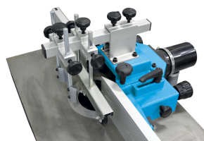
Guide with horizontal and vertical pressers
