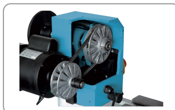
Variomatic speed control
