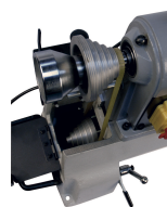
6 spindle speeds
