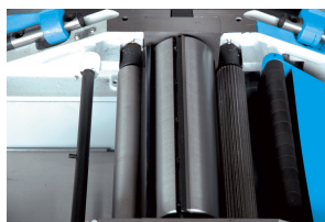
Driving rollers Ø 40 mm, 95 mm cutterblock with 4 blades
