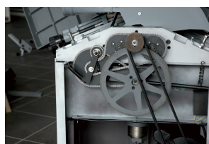
Rollers driven by chain, double-belt motor drive
