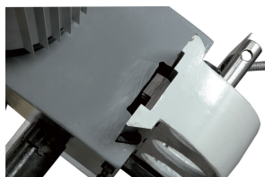
Sliding of head on dovetail
