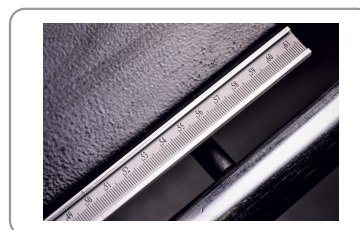
Rip fence with micrometric adjustment
